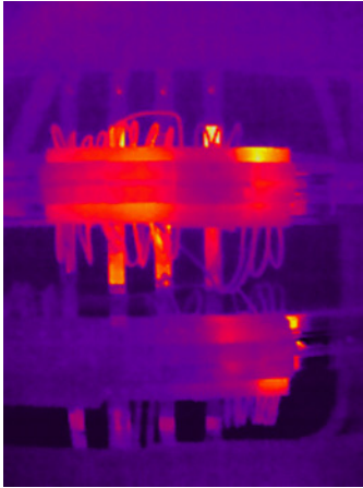
Electrical cabinets
