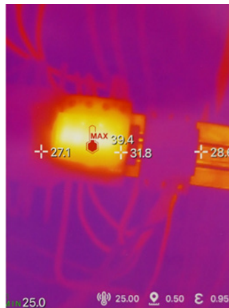
Electric switches
